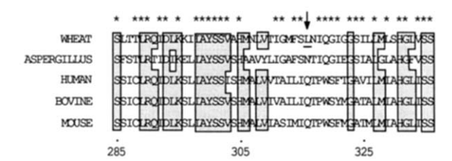
Fig.3. Comparison of part of the deduced amino acid sequence of the wheat mt NAD4 with the amino acid sequence of the corresponding protein from Aspergillus nidulans [20], human [21], bovine [22] and mouse [23] mitochondria. The arrow indicates the position of the leucine found at the E2-E3 junction. Stars indicate the homologies with the Aspergillus nidulans NAD4 amino acid sequence. Boxes indicate the homologies which exist in this part of the NAD4 protein between wheat and the other organisms.
